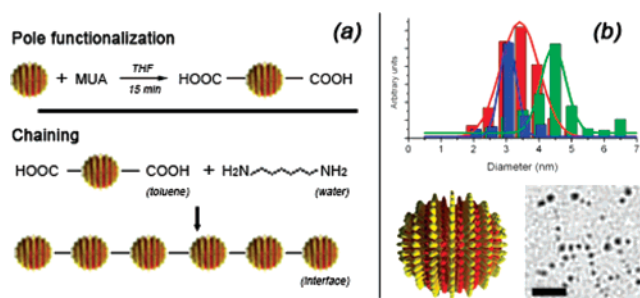
Figure 1. (a) Two steps of chain formation: pole functionalization of rippled NPs with MUA then interfacial polymerization. (b) NP size distributions measured from TEM images. Red is that of the starting NPs, green is that of chained NPs, and blue is that of unchained NPs. Bars represent the actual distribution; lines are Gaussian fits. The graphs are normalized for better visualization; the average NP size after chaining is 2.7 nm. Below left is a cartoon of a rippled NP; below right is a representative TEM image of NP chains, scale bar 25 nm.
