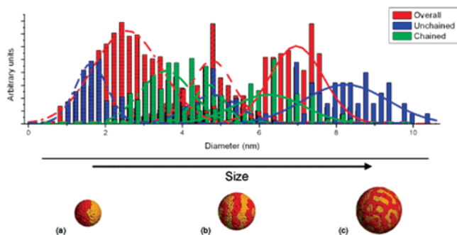
Figure 2. Size distributions before and after chaining for three different sets of NPs. Chains form only for NPs in a certain size range. Bars represent actual data; lines are Gaussian fits. Each type of line (solid, dashed, or dashed-dotted) represents one complete set of NPs (starting, unchained, and chained distributions). (a–c) Simulation snapshots of phase separation in mixtures of surfactants of unequal length on spheres of increasing diameter.
